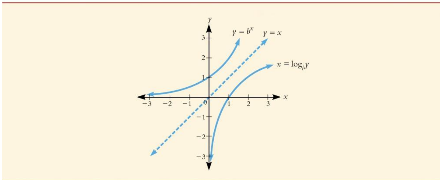
Figure 2.1 For example, if (0,1) is a point on the graph of an exponential function, then (1,0) would be the corresponding point on the graph of the inverse logarithmic function. (© S. A. Hummelbrunner)
