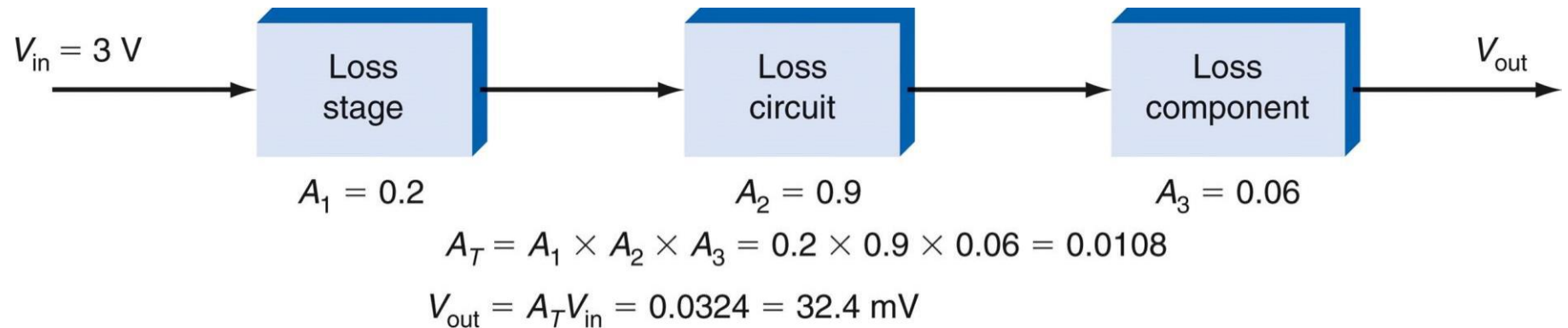
Figure 2-3: A voltage divider introduces attenuation.
